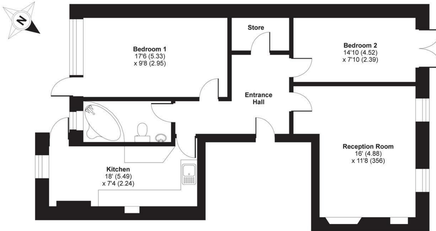
GROUND FLOOR
